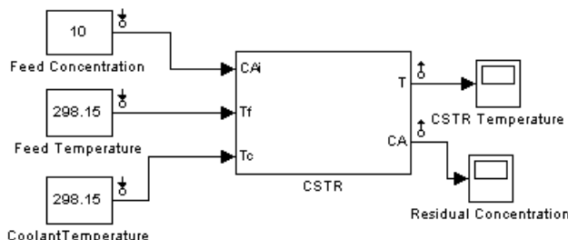
Figure 2-3: Simulink® Model of a Nonlinear Chemical Reactor
