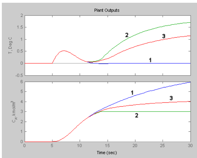
Figure 3-28: Constraint Softening Scenarios: 1 = None, 2 = Hard, 3 = Soft
